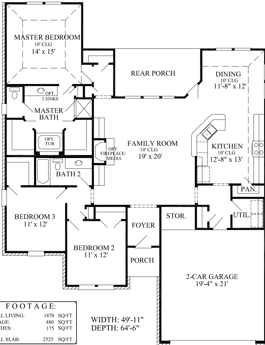
FLOOR PLAN
